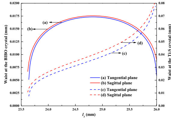
Fig. 2. Waist size at the center of the BIBO and Ti:S crystals as a function of the distance l_3 . (a) and (b), the waists at the BIBO crystal of the tangential and sagittal planes, respectively; (c) and (d), the waists at the Ti:S crystal of the tangential and sagittal planes, respectively.
